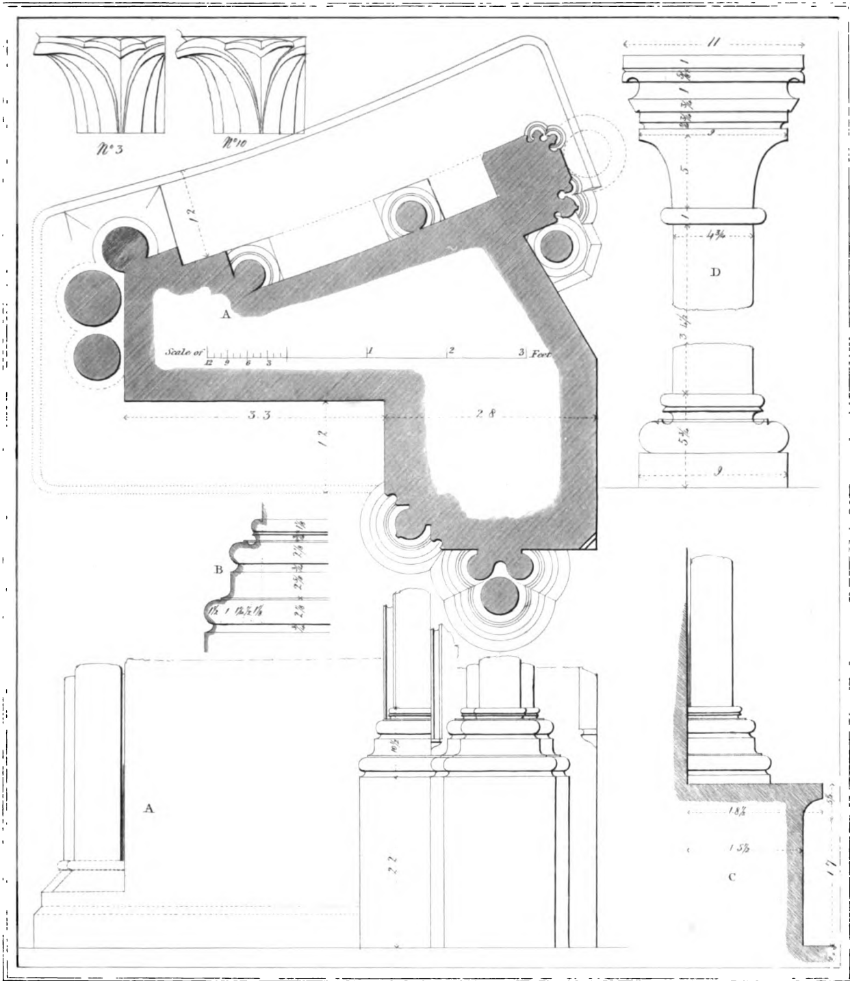
TEMPLE CHURCH, LONDON. DETAILS.
